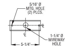
WALL CLEAT Mounting Hole Arrangement
